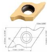
CARBIDE INDEXABLE INSERTS R2
